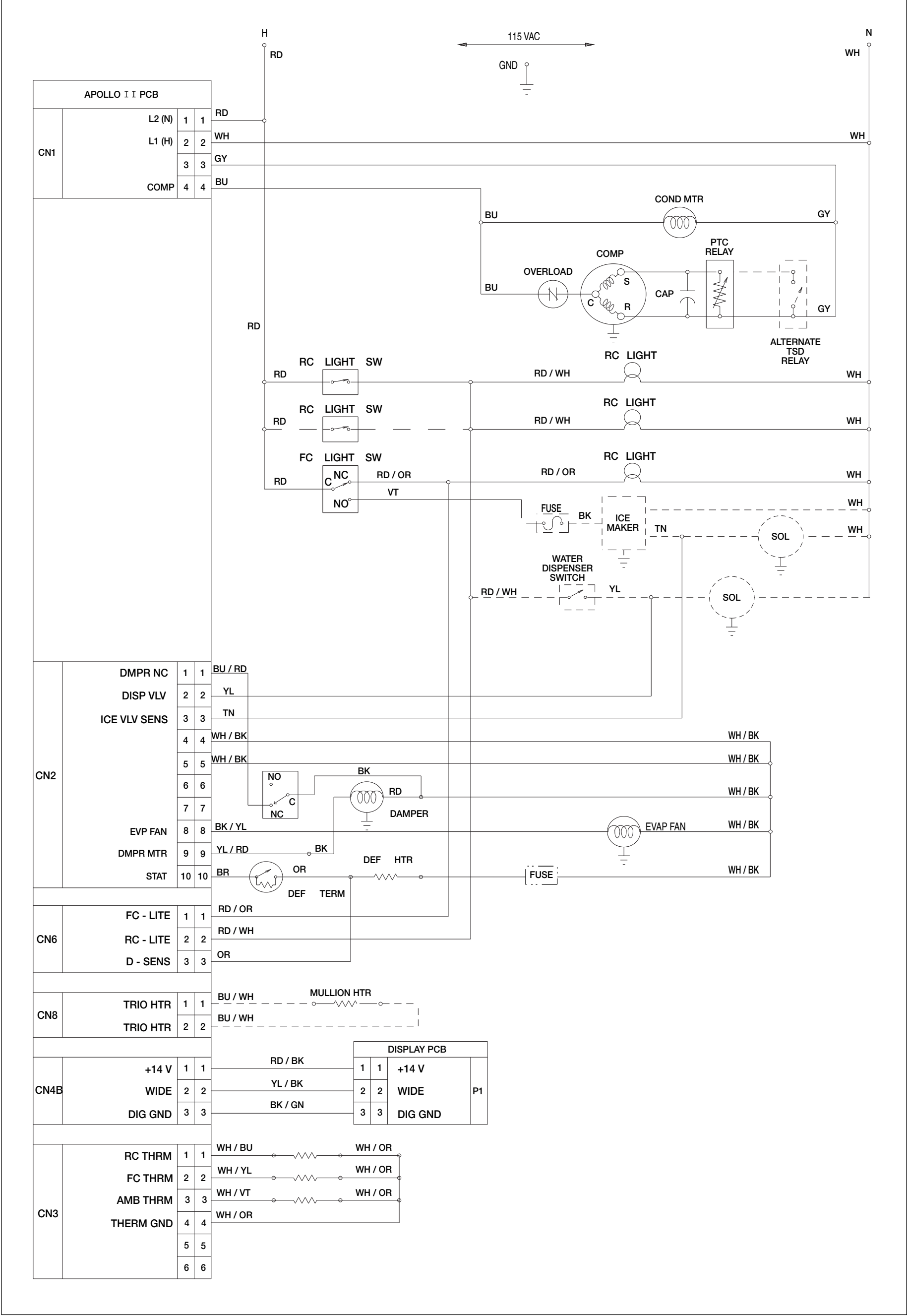
Schematic
