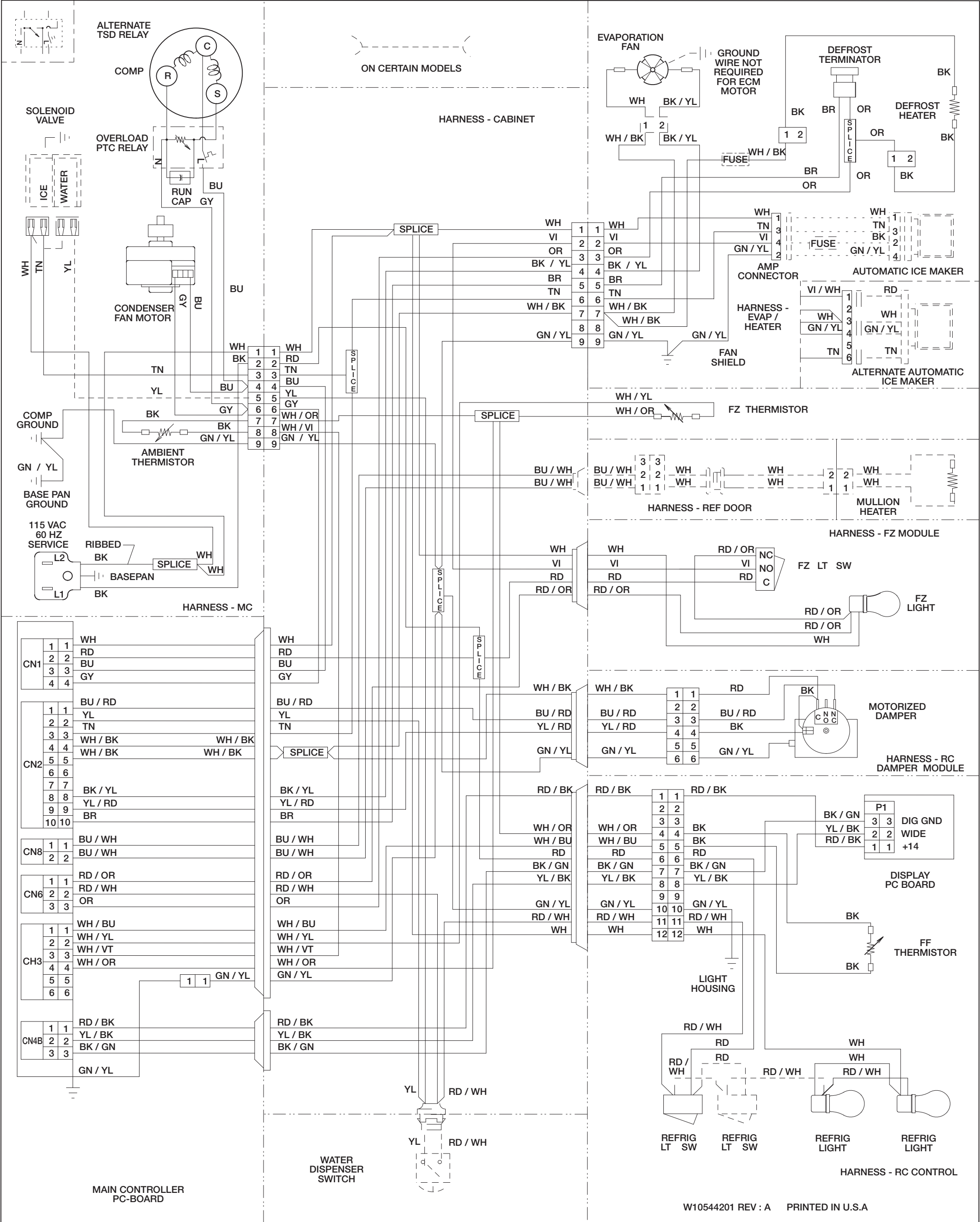
Wiring Diagram
