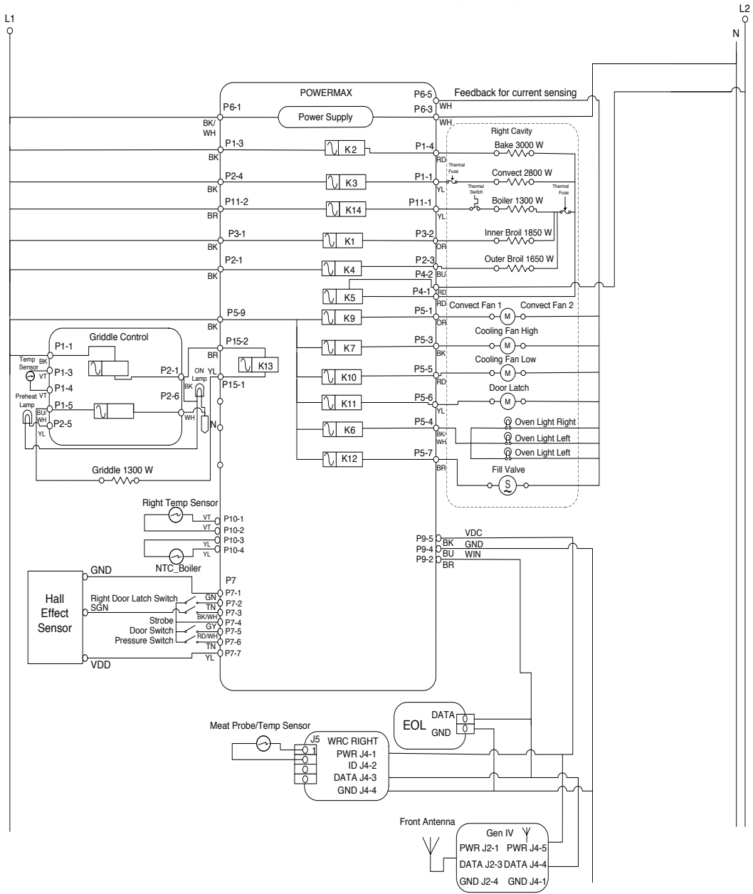
WIRE DIAGRAM Oven Control Wiring Diagram
