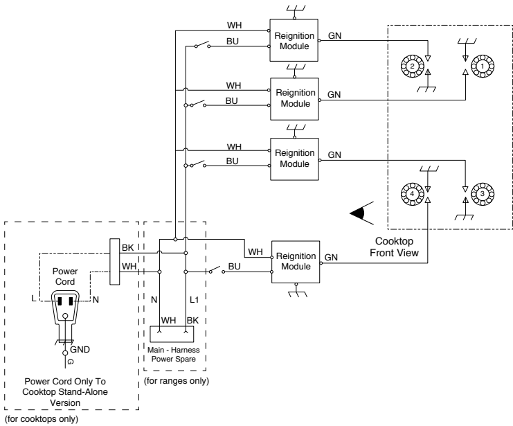
WIRE DIAGRAM - COOKTOP 4 Burner Cooktop
